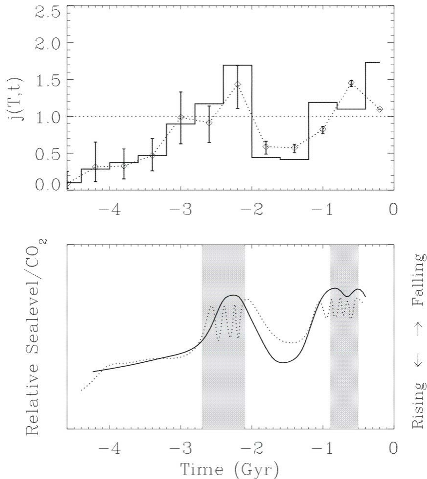
Figure 18. Top panel: Variation of Galactic Cosmic Ray (GCR) particles with energy 10 GeV at 1 AU over the entire history of the solar system. The error bars indicate the modulation for particles of 5 GeV (lower bound) or 20 GeV, respectively (upper bound). Lower panel: Generalized evolution of Earth's climate represented by relative sea level changes (solid curve) and relative changes of atmospheric content of \text{CO}_2 (dashed curve). The extremes indicate either a Greenhouse climate (Warm) or an Icehouse (Cold), corresponding to high sealevel/ \text{CO}_2 level or low sealevel/ \text{CO}_2 level respectively. The gray areas are known periods of glaciations.
