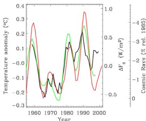
Figure 4: Tropospheric temperatures (black), obtained from radiosondes, shown together with reconstructed TSI (green), \Delta F_s , using re-scaled sunspot numbers as a proxy and cosmic rays (red). Both data sets have been low pass filtered with a three year running mean (adapted from Marsh and Svensmark, 2003b).
