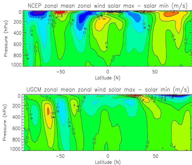
Figure 8: Differences in zonal wind speed between solar max and min from a) a multi regression analysis of NCEP reanalysis data between 1979-2002 and b) a GCM simulation (adapted from Haigh (1996) and Haigh et al. (2005)).
