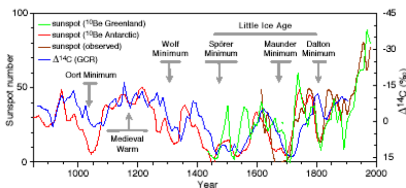
Figure 12: Changes in ^{14}\text{C} production relative to 1950 (blue) and reconstructed sunspot number from ^{10}\text{Be} for the past 1150 years. ^{14}\text{C} and ^{10}\text{Be} are produced through nuclear interactions of cosmic ray particles in the atmosphere. Cosmic rays are modulated by the solar wind; thus, variability in ^{14}\text{C} and ^{10}\text{Be} production is mainly a result of changes in solar activity. High solar activity leads to stronger shielding from the solar wind and thus a reduction in the production rate. Note the inverted axis for ^{14}\text{C} anomalies. The grey bars indicate major climate epochs. (adapted from Usoskin et al. (2003)).
