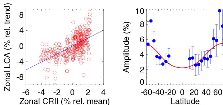
Figure 11: Latitudinal relation between relative variations of Low Cloud Amount ( LCA ) and Cosmic Ray Induced Ionisation ( CRII ) for the period 1984–2000 within the latitude range 55° – 20°S and 10°–70°N. a) Scatter plot of LCA vs. CRII , each dot representing an annual value within a 5° latitudinal bin. Solid blue line depicts the best linear. b) Latitudinal dependence of the amplitude of cyclic variations in LCA (blue dots) and CRII (red line). The amplitude is found by fitting a 10-year sinusoid to the respective time profiles. Adapted from Usoskin et al. (2004).
