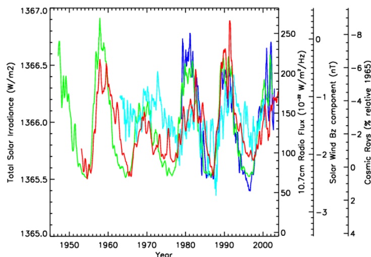
Figure 5: Monthly observations of TSI (blue) together with other solar parameters influencing Earth's environment: 10.7cm Radio Flux often used as a proxy for Solar UV (green), Solar Wind Bz component (light blue), and Cosmic Rays (red). All data have been smoothed with a 5-month running window.
