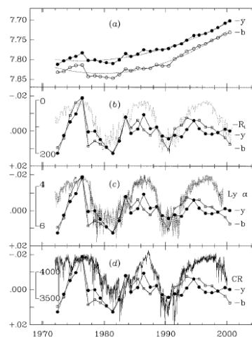
Figure 19: Neptune's brightness observed in band b (472-nm open dots) and band y (551-nm filled dots), correlated with solar activity. a) Neptune's brightness curve is fitted with a quadratic long-term trend, which is removed in the three remaining panels. Neptune's brightness anomalies (symbols) together with b) sunspot number, c) Lyman-a flux (a proxy for solar UV), and d) cosmic rays observed with the Climax neutron monitor (adapted from Lockwood and Thompson (2002) ).
