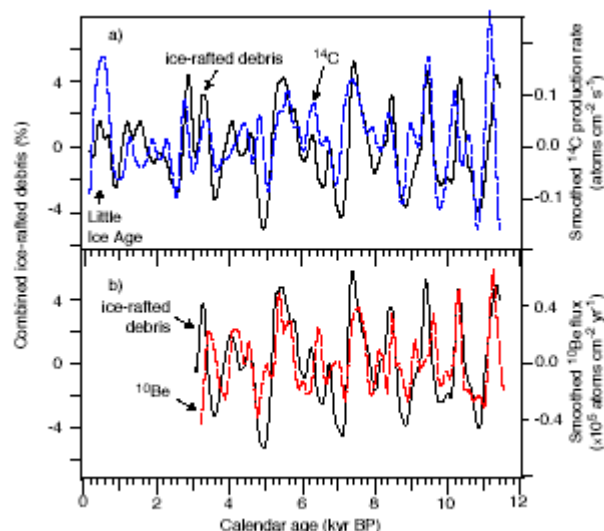
Figure 13: Correlation of ice-rafted debris from North Atlantic Ocean cores and solar activity indicated by a) ^{14}\text{C} and b) ^{10}\text{Be} (adapted from Bond et al. (2001)).
