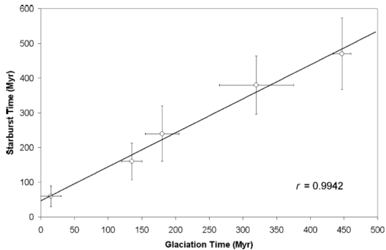
Figure 17: Enhanced star formation episodes as a function of the time-coincident glaciation events. A complete positive correlation is found within the error limits (adapted from de la Fuente Marcos and de la Fuente Marcos (2004)).
