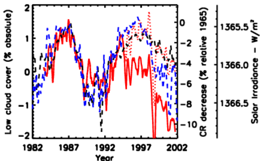
Figure 10: Monthly averages of ISCCP-D2 IR global Low Cloud Amount (red) shown together with cosmic rays (black dashed), and solar irradiance (blue dashed). The red dashed curve includes an offset after 1994 that has been added to Low Cloud Amount, this accounts for a possible inter-calibration problem at the end of 1994.
