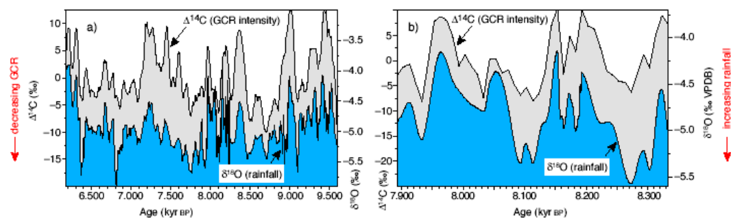
Figure 14: Profiles of \delta^{18}\text{O} from a stalagmite in Hoti cave, Oman, which is a proxy for monsoon rainfall, together with atmospheric ^{14}\text{C} obtained from Californian tree rings, which is a proxy for solar activity.
