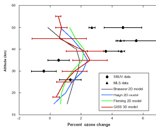
Figure 7: Annual average ozone differences between solar maximum and solar minimum between 60°S to 60°N in percent. Filled circles are from satellite observations covering 15 years for Solar Backscatter Ultraviolet (SBUV) data, and triangles are from 3 years for Microwave Limb Sounder (MLS) data. The coloured lines represent results obtained from various models of ozone photochemistry in the stratosphere (adapted from Shindell et al. (1999)).
