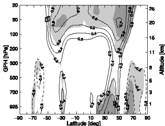
Figure 9: Linear correlations between the electric field of the solar wind and geopotential height variations as function of latitude at the zero meridian and geopotential height (adapted from Boberg and Lundstedt, 2003).
