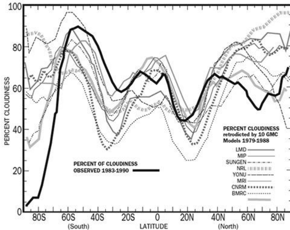
Figure 3. Heavy black line: observed cloudiness on Earth averaged over the years 1983–1990. Lighter and dotted lines: the average cloudiness on Earth over 1979–1988 as retrodicted by 10 revised General Circulation Models (GCMs). The GCMs identified by letter codes are detailed in Gates, et al. 24
