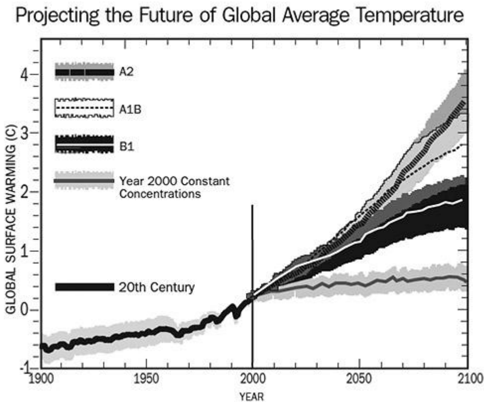
Figure 1. Projected increases in 21st century global average temperature assuming different \text{CO}_2 emissions futures (described below). These projections are from the 4AR Special Report on Emissions Scenarios (SRES), and appear in Figure SPM-5 of the Working Group I “Summary for Policymakers”. 11 The zero level was set to the average temperature between 1980–1999, which is why most of the 20th century shows negative values.
