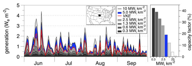
Fig. 1. (Left) Simulated daily mean electricity generation rates over the Kansas wind farm region (black square on map) for different installed capacities of up to 10 MW t ·km -2 . The higher installed capacities of 25 and 100 MW t ·km -2 are not shown, because they often yield less than the 10 MW t ·km -2 simulation. For comparison, the VKE estimate is shown in red. (Right) The mean per-turbine capacity factor derived for the different simulations.
