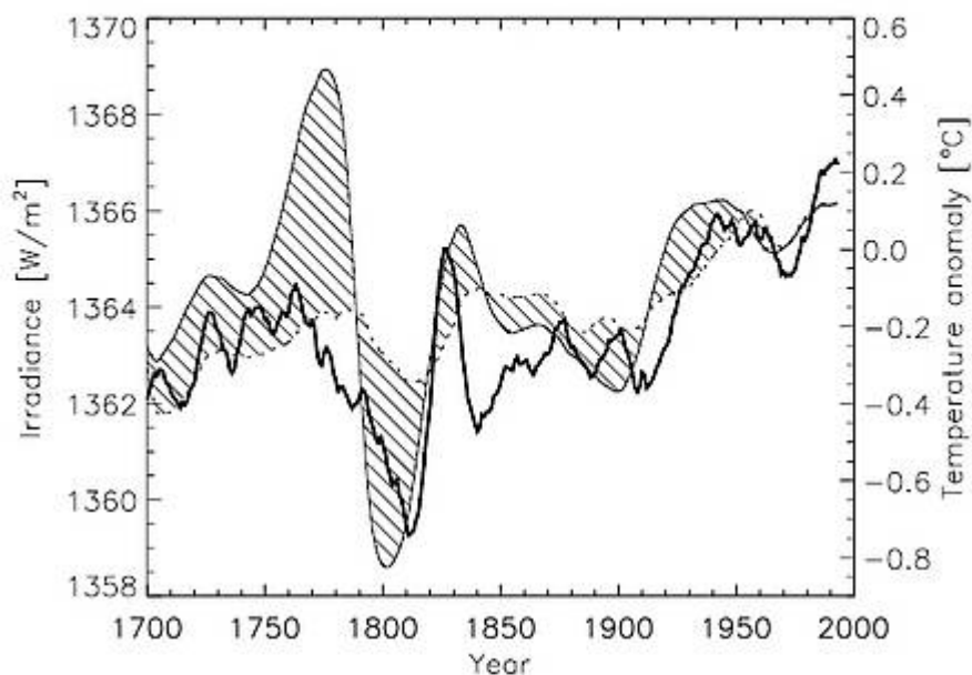
Figure 4. 11-year running mean of the two reconstructed S_{\text{rec}} . Thin solid curve: \Delta S_{\text{qs}} is represented by the solar cycle length; thin dashed curve: The amplitude of R_g is used as a proxy of \Delta S_{\text{qs}} . The hatched area gives a rough indication of the uncertainty in the reconstructions. Also plotted is the northern hemisphere land temperature (thick solid curve) according to Groveman and Landsberg (1700 – 1880) and the IPCC (1880 – 1990).
