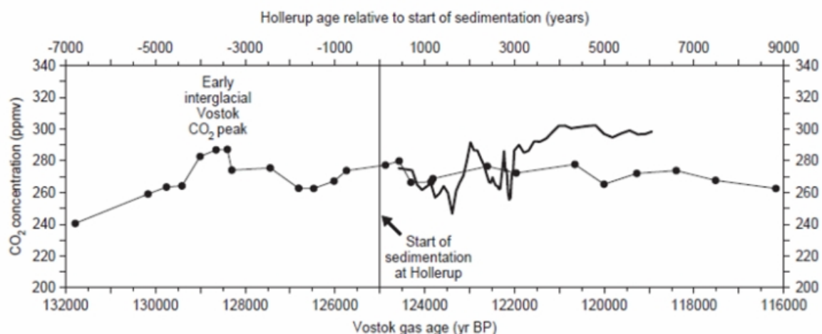
Fig. 5. Tentative matching of the Vostok \text{CO}_2 record (Petit et al., 1999) and Hollerup \text{CO}_2 reconstruction (five-point running mean values). The proposed matching takes into account the 6–7 kyr lag of peak interglacial sea levels relative to the early interglacial \text{CO}_2 peak in Vostok indicated by \delta^{18}\text{O}_{\text{atm}} measurements on atmospheric \text{O}_2 trapped in the Vostok core (Sowers et al., 1991) and the 3–4 kyr delayed attainment of maximum interglacial sea levels in the North Sea area relative to the onset of the Eemian in northwestern Europe (Zagwijn, 1996; Kristensen et al., 2000).
