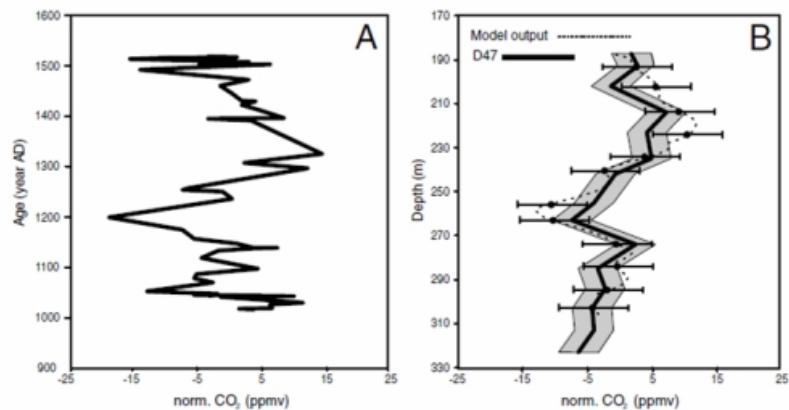
Fig. 1. (A) Raw data: normalized stomatal frequency based \text{CO}_2 mixing ratios as calculated from stomatal index: stomatal index (SI) (%) = [\text{stomatal density (SD) (number/mm}^2\text{)}]/[\text{stomatal density (SD) (number/mm}^2\text{)} + \text{epidermal cell density (ED) (number/mm}^2\text{)}] \times 100 of fossil Q. robur (oak) leaves derived from channel deposits of the River Roer (The Netherlands) (van Hoof, 2004; Wagner et al., 2004). The chronology of the stomatal frequency record is based on wiggle-match dating of eleven AMS ^{14}\text{C} measurements (van Hoof, 2004). (B) The dotted black line represents the \text{CO}_2 [SI] output after application of the firm densification model (Kaspers et al., 2004a). Of selected data points that resemble the actual sample depth of the \text{CO}_2 [ice] measurements of the D47 core, averaged errors of the \text{CO}_2 [SI] are shown. The black line represents normalized \text{CO}_2 mixing ratios ( \text{CO}_2 [ice]) of the D47 ice core and the grey area resembles the methodological error (Barnola et al., 1995).
