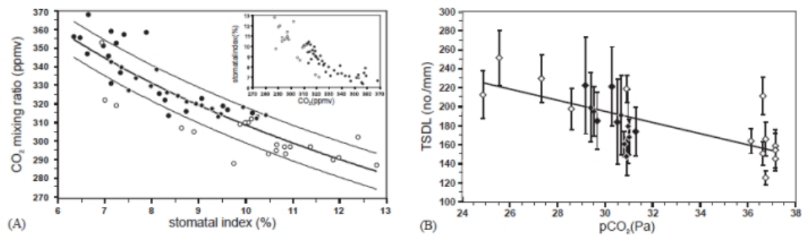
Fig. 1. Modelled relation between atmospheric \text{CO}_2 concentration and stomatal frequency in training sets consisting of leaves from herbaria and sub-fossil deposits calibrated against historical \text{CO}_2 concentrations. \text{CO}_2 mixing ratios of 290–315 ppmv were derived from shallow Antarctic ice cores ( http://www.cdiac.esd.ornl.gov/trends/co2/siple.htm ; Neftel et al., 1985), mixing ratios of 315–368 ppmv are annual means from instrumental measurements at Mauna Loa ( http://www.cdiac.esd.ornl.gov/ndps/ndp001.html ). (A) Thick black line: Model for \text{CO}_2 estimates based on linear regression of log-transformed stomatal index (SI) data for B. pendula pubescens ( \text{CO}_2 = 10^{2.802 - [0.313 + \log(\text{SI})]} ; r^2 = 0.79 ); thin lines indicate \pm 1 RMSE ( = 9.6 ppmv). Inset: historical response of SI to global atmospheric \text{CO}_2 . Training set includes leaf remains from modern peats (black circles) and herbarium specimens (open circles). (B) Response of number of stomata per millimetre needle length (TSDL) of T. heterophylla to a \text{pCO}_2 increase from 24 to 38 Pa. \text{CO}_2 partial pressure was calculated by multiplying the \text{CO}_2 mixing ratio by local barometric pressure P_B (Pa), estimated according to Jones (1992): P_B = 101.325 / e^{[(z/29.3)/T]} where z is the altitude above sea level and T the air temperature in K (estimated from mean annual temperature at the closest weather station, corrected by a temperature lapse rate appropriate for the region in case of significant altitudinal difference between site and station). Black diamonds represent sub-fossil and modern needles from Jay Bath (Mount Rainier, WA), open diamonds modern and herbarium needles from other localities. Error bars indicate \pm 1 SE. Solid line indicates best fit in classical regression analysis. TSDL: true stomatal density per millimetre needle length ( \text{TSDL} = -5.8581 \times \text{pCO}_2 + 371.14 ; r^2 = 0.5124 ; \text{RMSE} = 42.8 ppmv).
